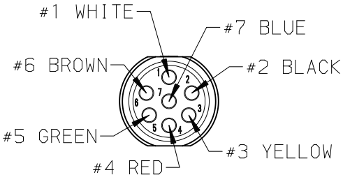
OPERATOR LOAD VIEW "B" (IN DIRECTION OF ARROW)
