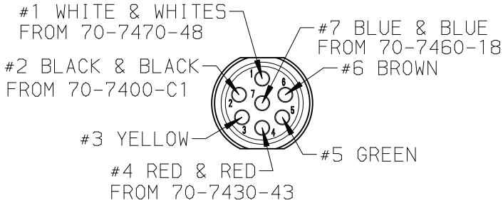
OPERATOR LOAD VIEW "A" (IN DIRECTION OF ARROW)
